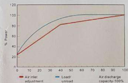
Part load performance
